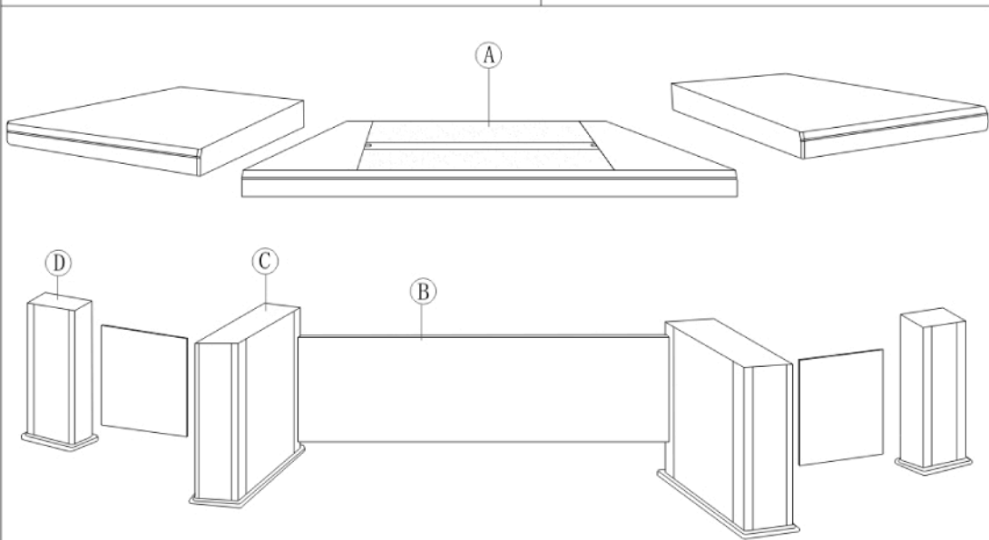
Exploded View:
